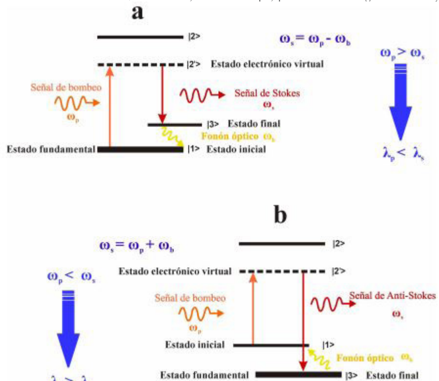
Figure 1. SRS process: (a) Stokes wave; (b) Anti-Stokes wave (Carrasco, 2007) / Proceso SRS: (a) Onda Stokes; (b) Onda Anti-Stokes (Carrasco, 2007)
